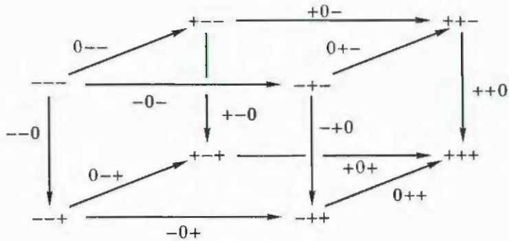
The 3-cube \mathbf{l}[3, 1] .
