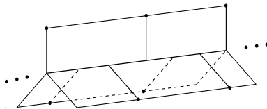
FIGURE 2. The universal covering space of X_m
